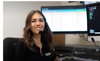
Graphic Editor
